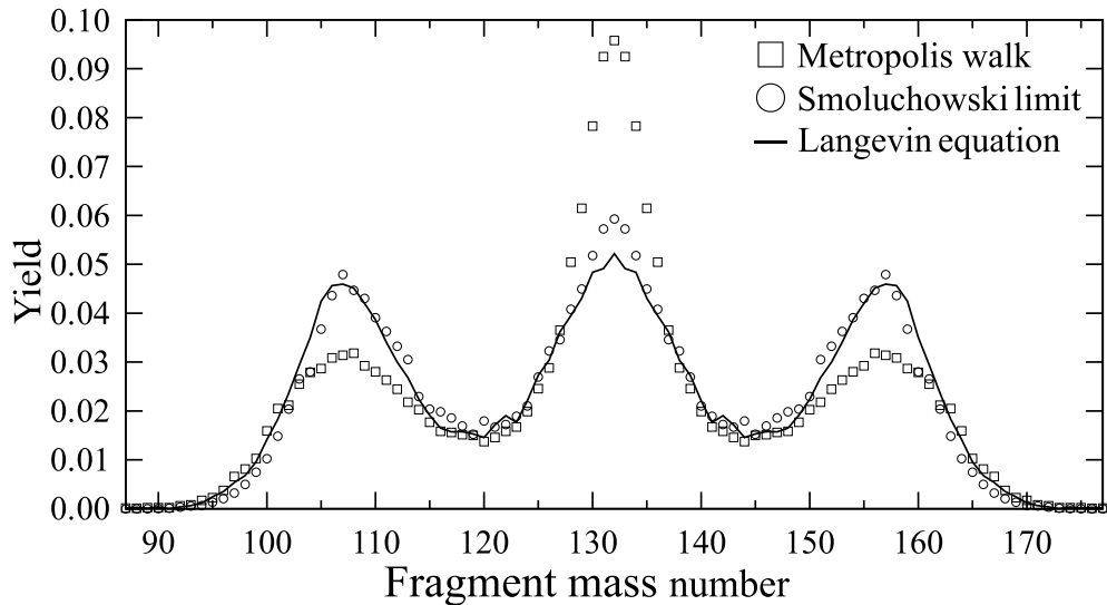
Figure 1. Calculated fragment mass distributions for fission of ^{264}\text{Fm} . Squares give the results using the Metropolis walk and circles give the results using the Smoluchowski limit. For clarity of the graph, the results using the Langevin equation are shown as a solid line.
