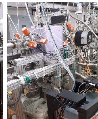
gas target
